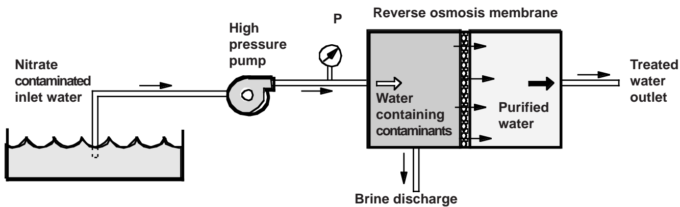
Figure 2. A schematic of the reverse osmosis process.
